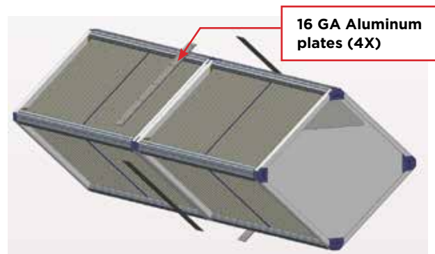
Figure 18 Joining sections (Completing the assembly)
