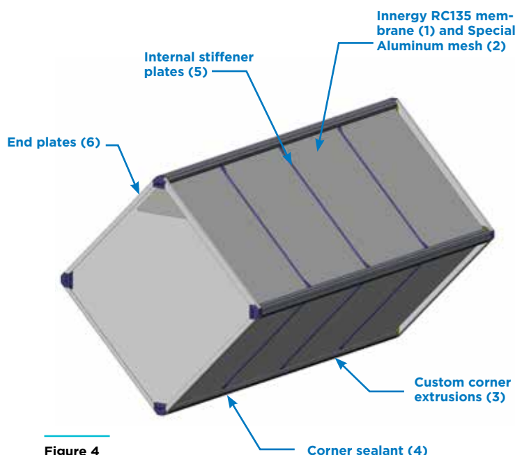
Figure 4 IPE5 main components
